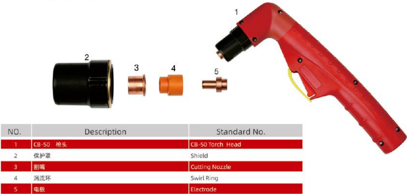
ORK CB-50 Air Cooled Plasma Cutting orch ORK CB-50 气体冷却等离子切割枪
