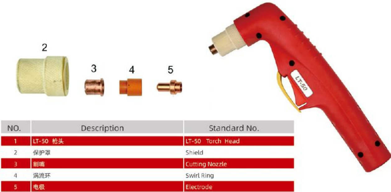
ORK LT-50 Air Cooled Plasma Cutting Orch ORK LT-50气体冷却等离子切割枪
