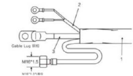
WP-26,WP- 26F ,WP- 26V,WP- 26FV,WP-26P Torch Terminations(Cable and Gas Separate) WP-26 系列焊枪接口 (气电分体)
