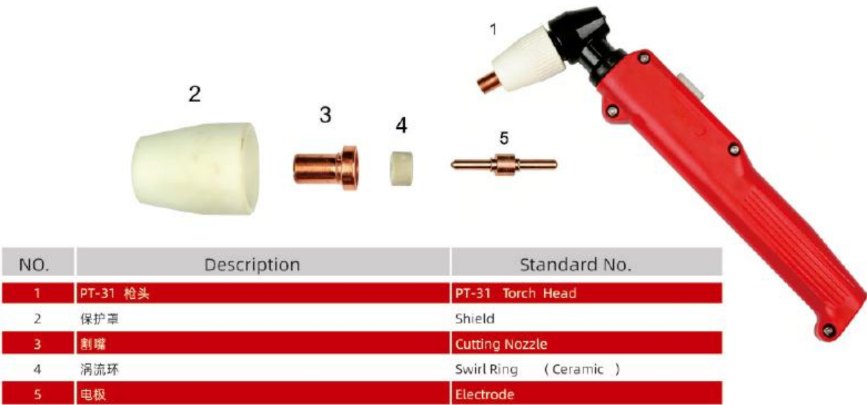
ORK PT-31 Air Cooled Plasma Cutting orch ORK PT-31 气体冷却等离子切割枪
