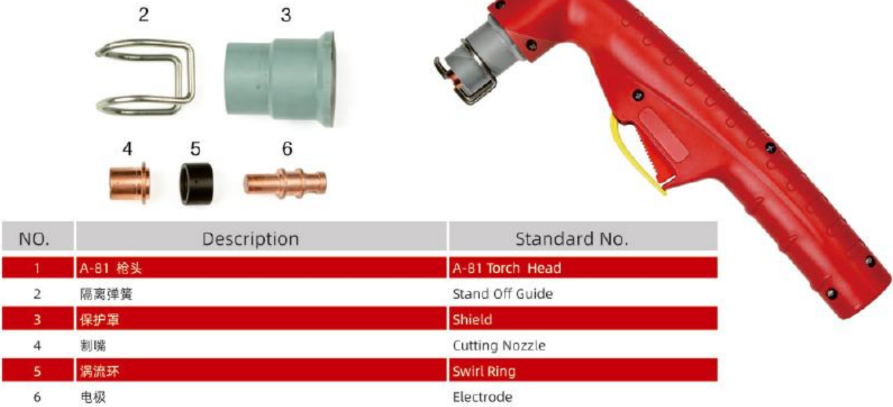
ORK A-81 Air Cooled Plasma Cutting orch ORK A-81 气体冷却等离子切割枪
